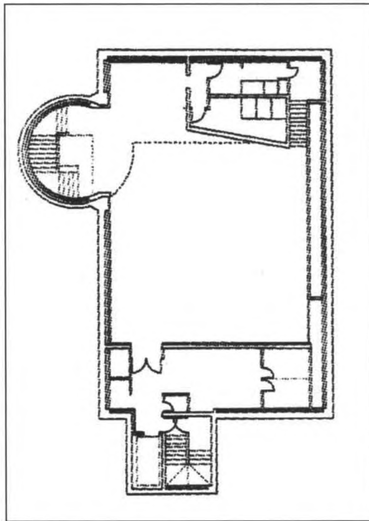
Fig. 17: Phase V showing lower level plan. (Source: Maki and Associates, On Maki Architecture/Maki on Architecture , Tokyo, Fumihiko Maki Traveling Exhibition Executive Committee, 2001, p. 21).
